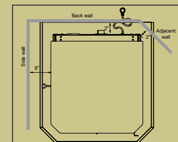
Figure 4. Minimum Clearances to Combustibles for Freestanding Kinderhook.
